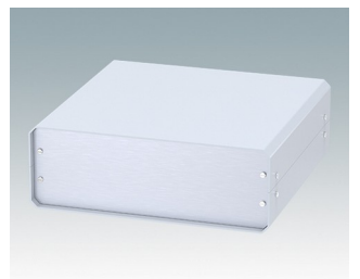
M5502110 UNICASE 2 Aluminium Light grey RAL 7035 260x250x90mm
